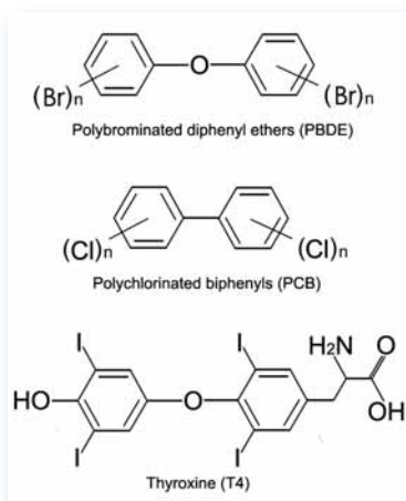
Figure 6 Chemical structure of PBDEs, PCBs and thyroxine ( T_4 ). The similarity of PBDEs and PCBs to thyroid hormones may underlie the chemicals' toxicity. All of the compounds consist of two six-carbon rings decorated with halogens. Bromine attaches to the carbon rings of PBDEs, chlorine to those of PCBs, and iodine to those of thyroid hormone. In PBDEs, an atom of oxygen bridges the rings, whereas the rings of PCBs and thyroid hormones are linked by carbon-carbon bonds
